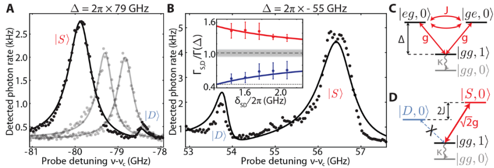
Fig. 2. Cavity mediated SiV-SiV interactions. (A) Transmission spectrum of two nearly-resonant SiVs ( \delta = 2\pi \times 0.56\text{GHz} ) at cavity detuning ( \Delta = 2\pi \times 79\text{GHz} ). When both SiVs are coupled to the cavity, superradiant (bright) |S\rangle and subradiant (dark) |D\rangle states are formed (black). Spectra of non-interacting SiVs are shown in gray. (B) Transmission spectrum of the same SiVs at \Delta = 2\pi \times -55\text{GHz} and \delta = 2\pi \times 2\text{GHz} . Inset: ratio of |S\rangle (red) and |D\rangle (blue) state linewidths to the single-SiV linewidth at ( \Delta = 2\pi \times 79\text{GHz} ) as a function of \delta_{SD} . The resonance frequencies of these SiVs slowly drift due to spectral diffusion (14), allowing us to measure the linewidths of |S\rangle and |D\rangle at different \delta_{SD} . The gray dashed line and shaded region are the average and standard deviation of the single-SiV linewidths. The dotted line corresponds to the SiV linewidth \gamma without Purcell enhancement, demonstrating that |D\rangle at minimum \delta_{SD} is almost completely decoupled from the cavity. Solid lines in (A) and (B) are predictions based on independently-measured SiV parameters (16). (C) Energy diagram of two SiV centers coupled to a cavity mode. Interaction via exchange of cavity photons at rate J = g^2 / \Delta leads to collective |S\rangle and |D\rangle eigenstates (D).
