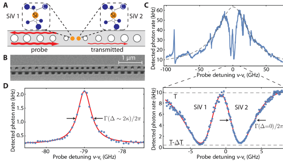
Fig. 1. High cooperativity SiV-photon interface. (A) Schematic of a diamond nanocavity containing two SiV centers. (B) Scanning electron micrograph of a nanocavity. (C) Transmission spectrum of the coupled SiV-cavity system (blue). The broad Lorentzian response of an empty cavity (dashed) is modulated by cavity-coupled SiVs. Near the cavity resonance (lower panel), two SiVs each result in greater than 95% extinction in transmission and are broadened by the Purcell effect ( \Gamma(\Delta=0) = 2\pi \times 4.6\text{GHz} ). (D) In the dispersive regime ( \Delta = 2\pi \times 79\text{GHz} \sim 2\kappa ), SiVs appear as narrow peaks in transmission ( \Gamma(\Delta) = 2\pi \times 0.5\text{GHz} ). The solid lines in (D) and the lower panel of (C) are fits to a model (16).
