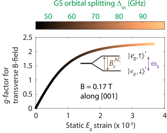
FIG. 10. g -factor for a transverse microwave magnetic field resonantly driving the spin qubit (interaction shown in inset) calculated as a function of pre-existing static E_g -strain plotted along x -axis. Color variation along the curve shows the GS splitting corresponding to the value of static E_g -strain at the SiV. Both the DC and AC strain are assumed to be entirely in the E_{gx} -component.
