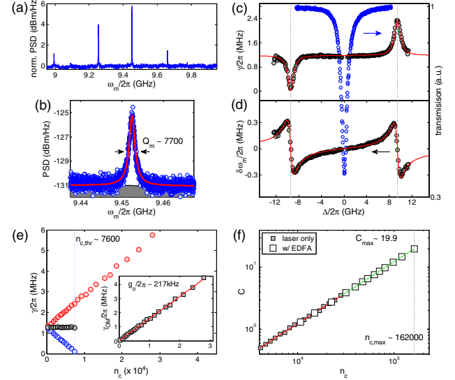
Fig. 5. Acoustic swelling mode mechanical spectroscopy. (a) Normalized power spectral density revealing a zoomed-in radio frequency spectrum of optically transduced diamond OMC thermal Brownian motion near \sim 9.5 \text{ GHz} . (b) High-resolution PSD of the diamond OMC acoustic “swelling” mode centered at \omega_m/2\pi = 9.454 \text{ GHz} . The Lorentzian fit (solid red curve) estimates a Q_m \sim 7700 , corresponding to an f \cdot Q product of \sim 7.3 \times 10^{13} \text{ Hz} . The (c) optically amplified mechanical loss rate and (d) optical spring-shifted mechanical frequency measured as a function of the laser detuning frequency at a constant intracavity photon number of n_c = 6000 . The optical transmission spectrum (blue circles) is also plotted, with vertical gray dashed lines indicating \Delta = \pm \omega_m . Fits to (c) and (d) (red solid lines) yield estimates of \gamma_i/2\pi = 1.18 \text{ MHz} and g_o/2\pi = 239 \text{ kHz} . (e) Measured mechanical linewidths ( \gamma ) collected at laser detuning of \Delta = +\omega_m (red circles) and \Delta = -\omega_m (blue circles). Gray circles, which indicate the intrinsic mechanical linewidth values ( \gamma_i ) obtained by taking the average of the detuned data, yield an estimate of \gamma_i/2\pi = 1.27 \pm 0.02 \text{ MHz} . The inset displays calculated optomechanically induced damping ( \gamma_{OM} = \gamma_{red} - \gamma_i , black squares), plotted versus intracavity photon number ( n_c ). A linear fit (red solid line) yields g_o/2\pi = 217 \pm 12 \text{ kHz} . Under blue laser detuning, an threshold input power of n_{c,\text{thr}} \sim 7,600 (vertical blue dashed line) is required to observe phonon lasing of the mechanical cavity. (f) Cooperativity values ( C \equiv \gamma_{OM}/\gamma_i ) collected under red laser detuning, plotted versus n_c . Solid gray squares and the linear fit (solid red line) are calculated from the \gamma_{OM} values shown the panel (e) inset. Open gray squares correspond to mechanical spectra collected with the input laser amplified by an erbium doped fiber amplifier. The extrapolated linear fit (dashed green line) was used to infer the corresponding n_c values. A maximum cooperativity value of C \sim 19.9 was measured at an estimated n_c \sim 162,000 (vertical dashed gray line).
