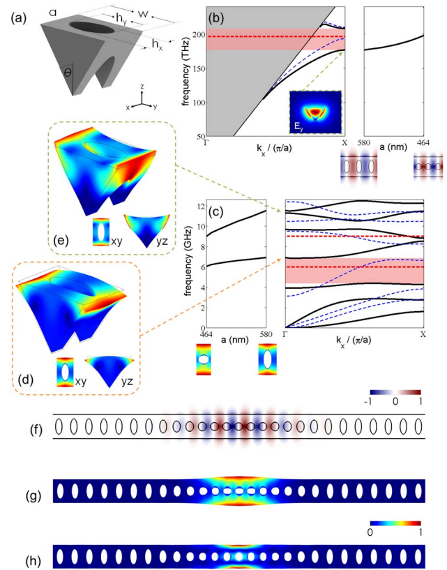
Fig. 1. Diamond optomechanical crystal optimized design. (a) Solid model representation of the triangular cross-section unit cell, which is parameterized by the etch angle ( \theta ), width ( w ), lattice constant ( a ), and elliptical air hole diameters ( h_x, h_y ). Corresponding (b) optical and (c) mechanical band structures of a nominal diamond unit cell with \theta = 35^\circ and (a, w, h_x, h_y) = (580, 929, 250, 590) nm. Below the light line in (b), supported transverse electric (TE-like) and transverse magnetic (TM-like) guided modes are indicated by solid black and dashed blue lines, respectively. The left panel inset of (b) displays the cross-sectional optical E_y -field profile of the first (dielectric) TE-like guided optical mode at the X-point. In (c), mechanical guided modes shown are for propagation along the x -axis, with y -symmetric and y -antisymmetric vector symmetries again indicated by solid black and dashed blue lines, respectively. Mechanical simulations assume guided mode propagation is oriented with the in-plane [110] crystallographic direction, with the z -axis oriented along [001]. The pink shaded regions in (b) and (c) highlight the optical and mechanical symmetry bandgaps of interest, respectively. Three-dimensional mechanical displacement profiles of the acoustic (d) “flapping” and (e) “swelling” guided modes originating from the \Gamma -point of the fourth and seventh y -symmetric bands, respectively. The right and left panels in (b) and (c), respectively, show the tuning of the X-point optical and \Gamma -point mechanical modes of interest as the unit cell is transitioned smoothly from the nominal unit cell to a defect cell with a reduced lattice constant and decreased air hole eccentricity, specifically, (a_{\text{defect}}, h_{x,\text{defect}}, h_{y,\text{defect}}) = (464, 327, 289) nm. Normalized (e) optical E_y -field of the localized optical cavity mode and mechanical displacement profiles of the (f) flapping and (g) swelling mechanical cavity modes for the optimized diamond OMC design. Eigenfrequencies of these localized optical and mechanical modes are indicated on the respective band structures in (b) and (c) by dashed red lines.
