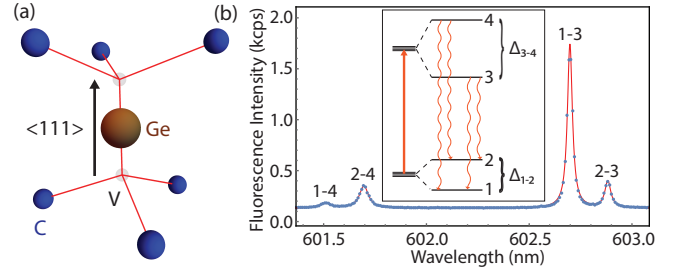
FIG. 1. (a) Molecular structure of the GeV center. (b) Photoluminescence spectrum of the GeV at T = 50 K, revealing the four optical transitions predicted by the GeV electronic structure (inset) [13]. \Delta_{1-2} = 152 GHz and \Delta_{3-4} = 981 GHz are the measured ground and excited state orbital splittings respectively. The solid curve is a fit to four Lorentzians.
