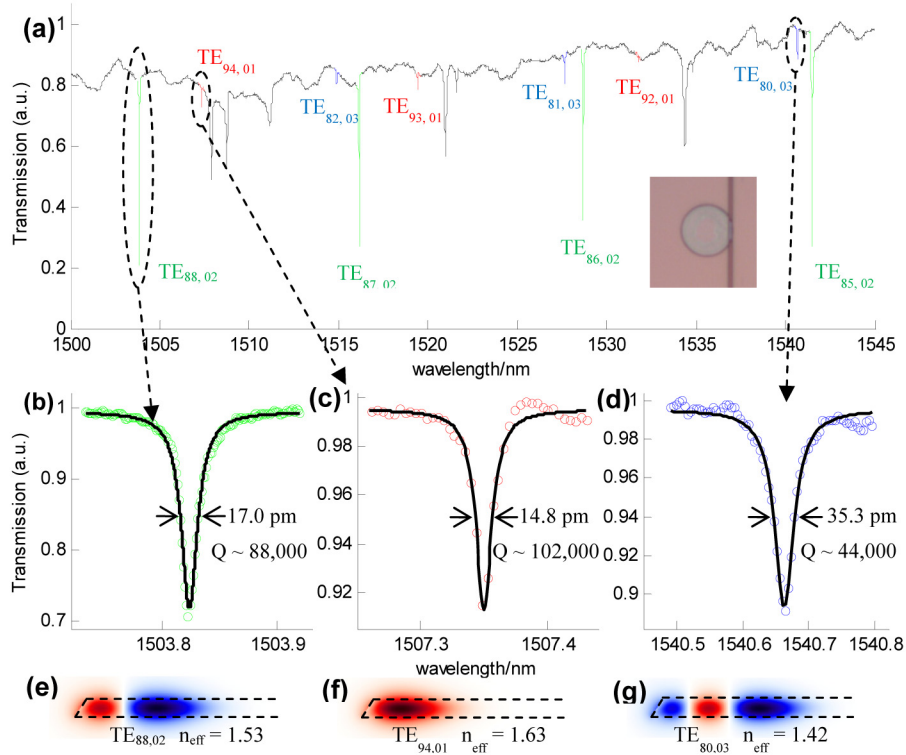
Fig. 2. Resonance spectra and simulation results in telecom wavelengths. (a) A representative transmission spectrum collected from a 28 \mu\text{m} diameter disk revealing several sets of resonances, indicated by color coding. Each resonant dip is labeled as \text{TE}_{mn} , where m, n are the azimuthal and radial mode numbers respectively. Inset shows the optical micrograph of tapered fiber coupling on top of the microdisk resonator. (b-d) High-resolution views of representative resonance dips for each radial mode and their corresponding Lorentzian fits (black curves), indicating quality factors of 1.02 \times 10^5 , 8.8 \times 10^4 and 4.4 \times 10^4 for 1st (c), 2nd (b) and 3rd (d) order radial modes respectively. (e-g) Finite element mode simulation of the three radial order modes shown in (b-d), indicating TE-like modes. Electric fields along radial direction ( E_r ) are shown, labeled with mode numbers and effective indices. Dashed lines show the outlines of the device cross section.
