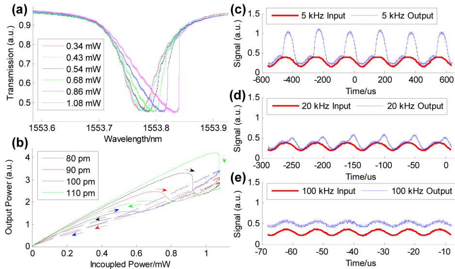
Fig. 5. Optical bistability and its time-domain response. (a) Transmission spectra of a LN microdisk resonance at different in-coupled power levels, showing red-shift of resonant frequency and optical bistability at elevated input power. The baselines of each spectrum are normalized by input power. (b) Power hysteresis curves at different red-detuned laser wavelengths (legend indicates detuning). The arrows show the directions to which the laser power is swept. (c-e) Time-domain power responses showing both input optical signals (red) and output detector signals (blue) at different modulation frequencies: (c) 5 kHz, (d) 20 kHz and (e) 100 kHz.
