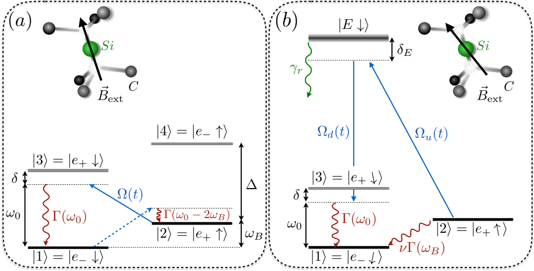
FIG. 1: Comparison of the two driving schemes to implement the spin-phonon interface. (a) A microwave magnetic field drives the transition |2\rangle \rightarrow |3\rangle , and state |3\rangle subsequently decays to state |1\rangle by emitting a propagating phonon at frequency \omega_0 . The process that drives the transition |1\rangle \rightarrow |4\rangle is strongly off-resonant for large Zeeman energy \omega_B \gg \delta and can be neglected. (b) The transition |2\rangle \rightarrow |3\rangle is now driven by two optical fields via the excited state |e_u \downarrow\rangle of the SiV center. In that case, the external magnetic field has to be tilted from the symmetry axis of the defect. As a consequence, it opens a decoherence channel via the direct transition |2\rangle \rightarrow |1\rangle .
