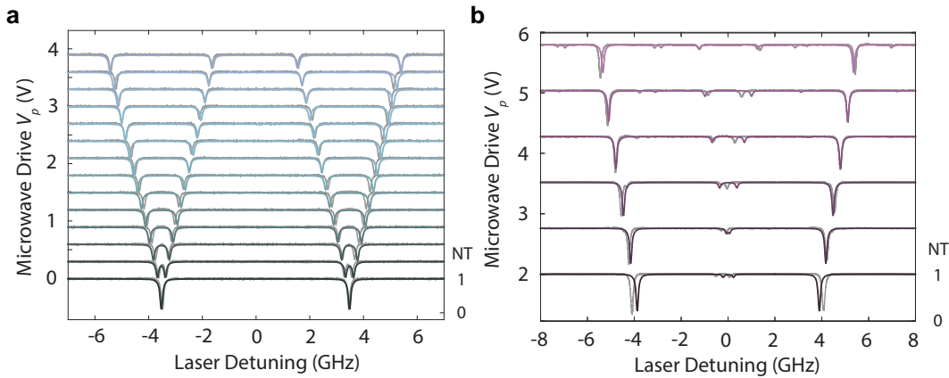
FIG. S-4: Calculated optical transmission spectrum for Autler-Townes (AT) splitting and AC Stark shift a , Colored curves: simulated AT spectrum with full mode described in eqn S-2. Gray curves: experimental data as shown in Fig. 2 in the main text. b , Colored curves: simulated AC Stark shift spectrum with full mode described in eqn S-2. Gray curves: experimental data.
